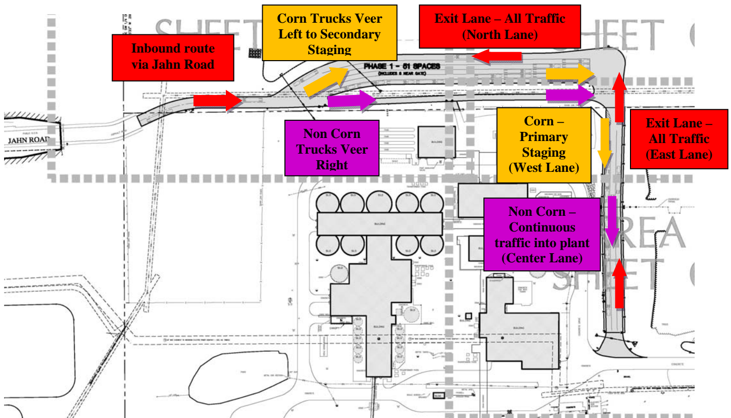
Figure B – Truck Traffic Patterns Through New Staging Area
