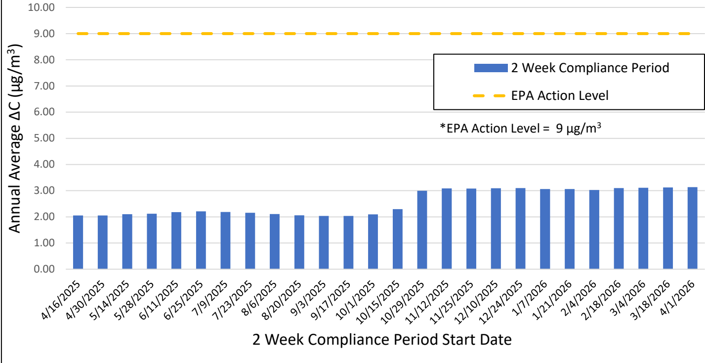
BENZENE FENCELINE ROLLING ANNUAL AVERAGE CONCENTRATION 04/16/2025 -04/15/2026
